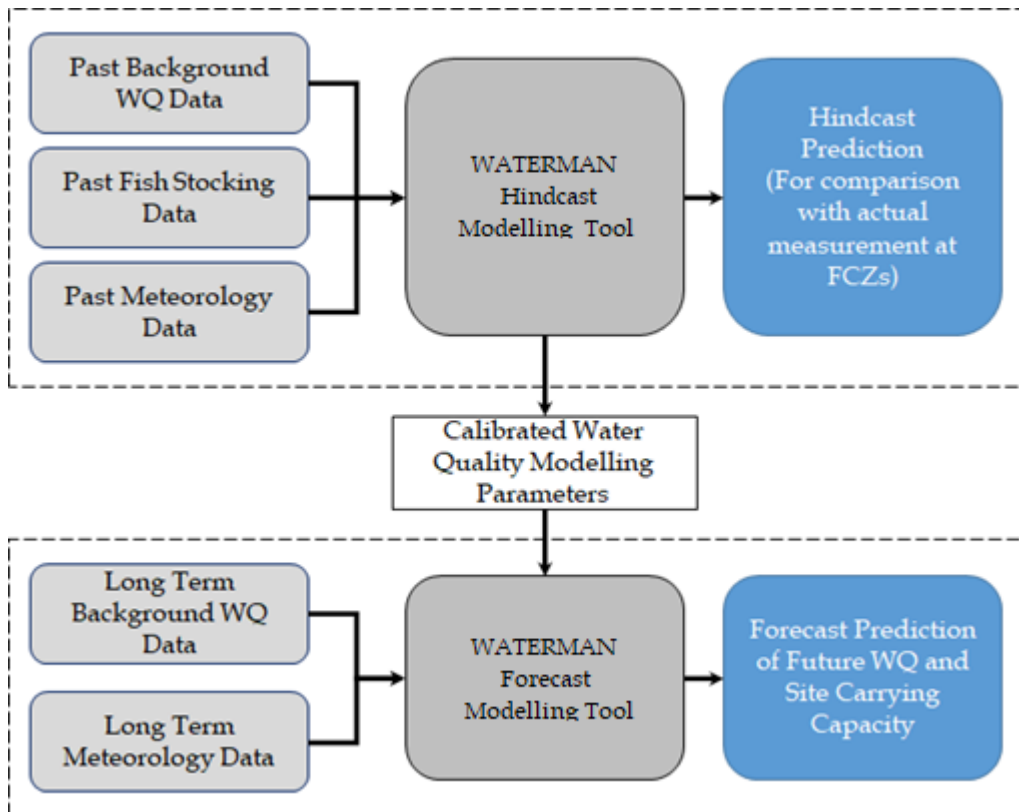
Figure 3.4 Relationship of the WATERMAN Hindcast and Forecast Modelling Tool
