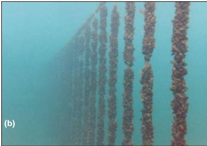
Figure 2.9 Examples of (a) Lantern Nets and (b) Longlines for Bivalve Culture (Source: Qingdao Mansheng Industry and Trade Co., Ltd., Department of Fisheries and Oceans)
