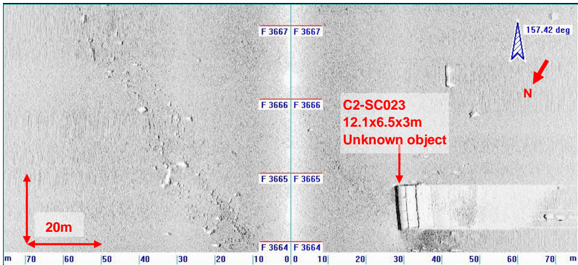
Figure 10.7 SSS Rectified Images Showing Sonar Contact C2-SC023 from Different Survey Lines in Site C2
