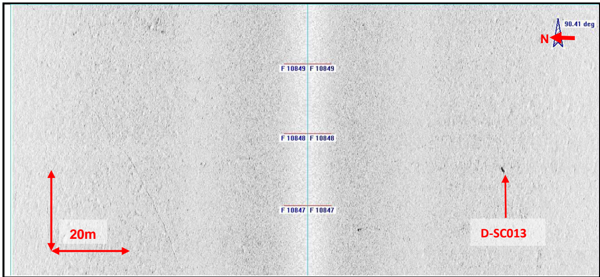
Figure 8.8 SSS Rectified Image Showing Sonar Contacts D-SC013
