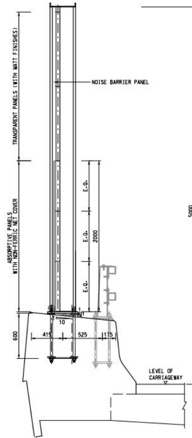
TYPICAL SECTION OF REPROVISIONED NOISE BARRIER (5m HIGH) AT LFRSR S/B
