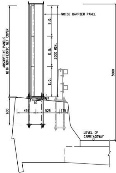
TYPICAL SECTION OF REPROVISIONED NOISE BARRIER (3m HIGH) AT LFRSR N/B
