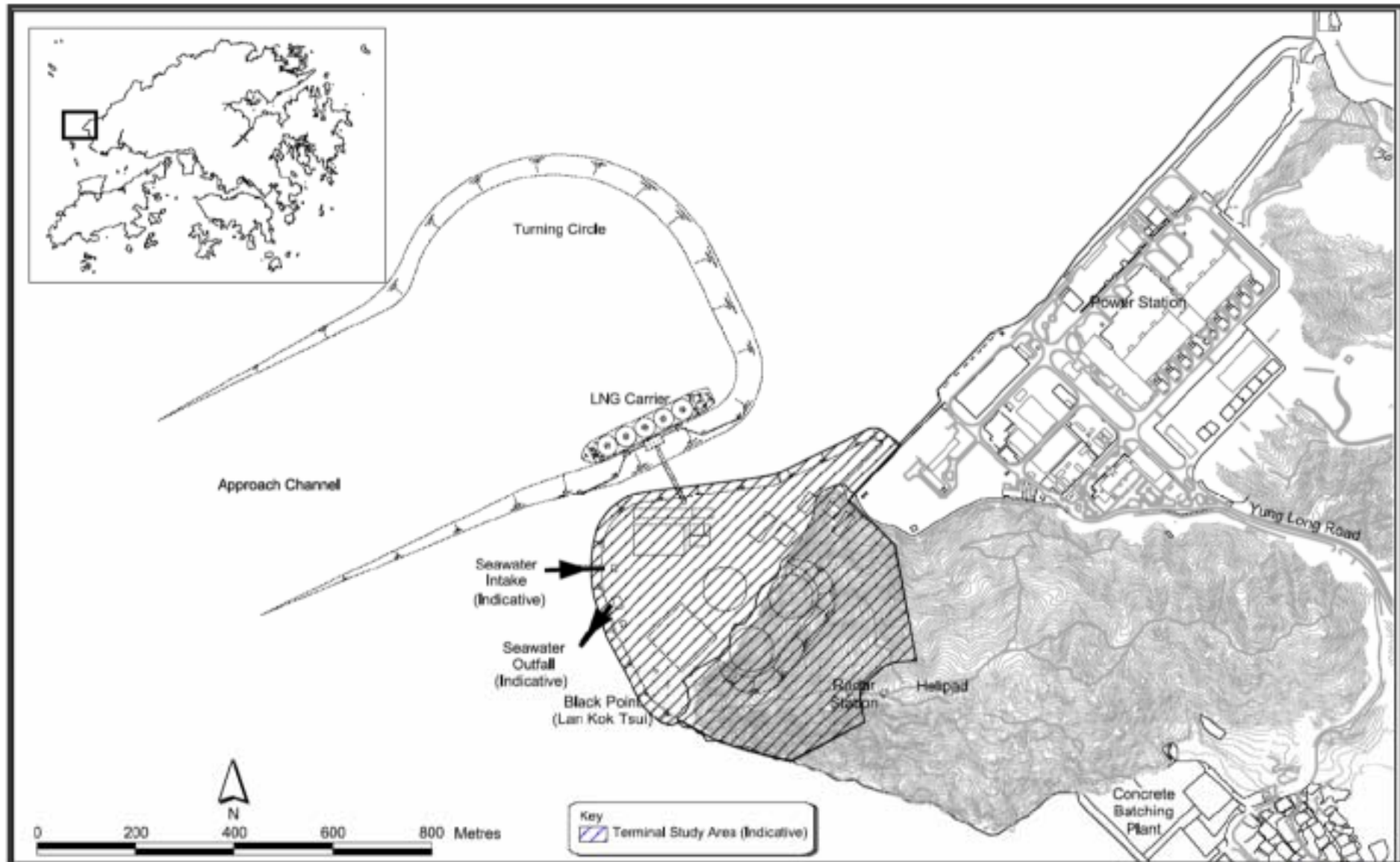
Appendix A2: Preliminary Conceptual Layout of Black Point LNG Terminal Project: Liquefied Natural Gas (LNG) Receiving Terminal and Associated Facilities ( Plan originated from Figure 2.4e of Project Profile )
