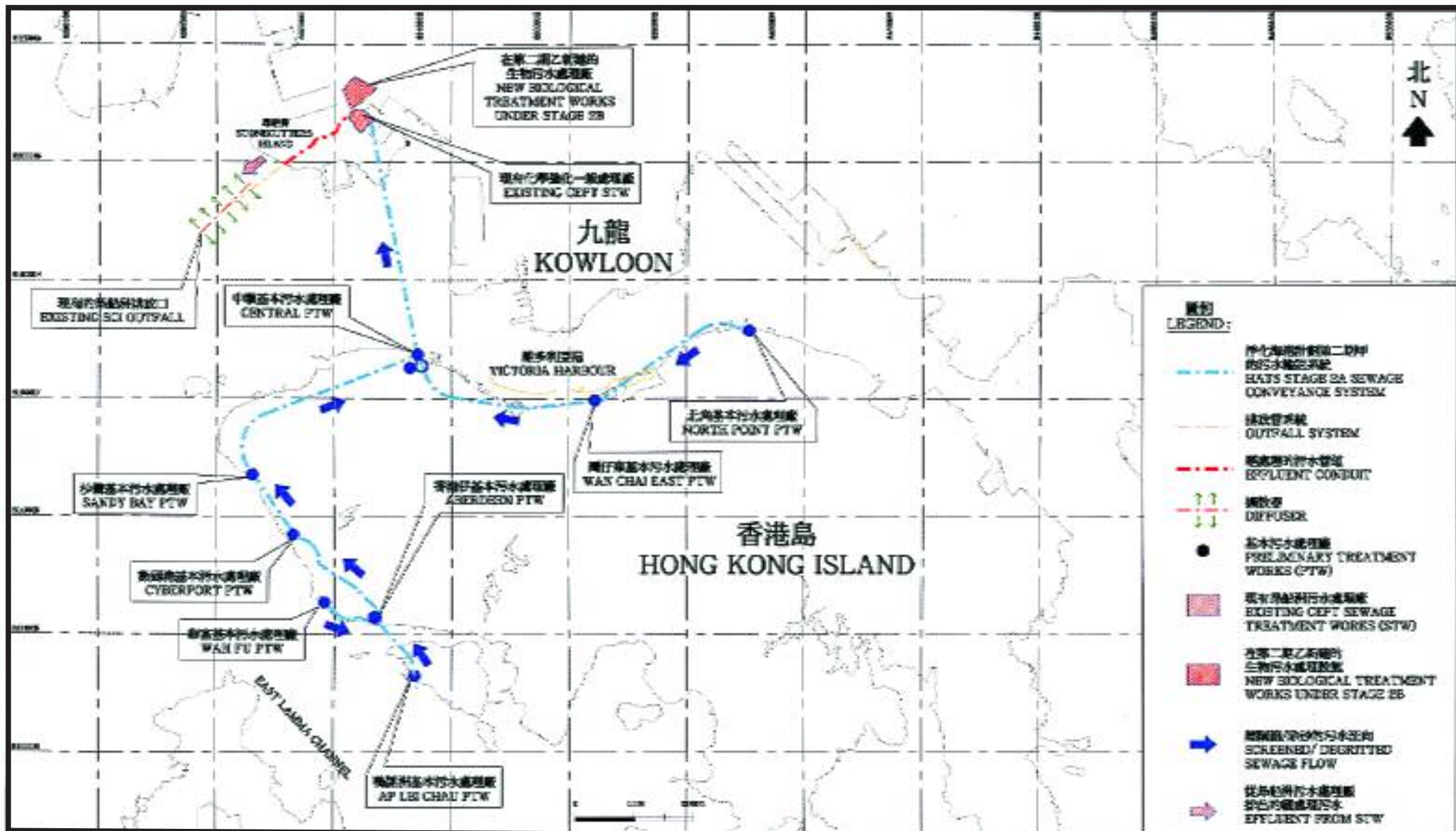
淨化海港計劃第二期 整體規劃圖 HARBOUR AREA TREATMENT SCHEME STAGE 2 OVERALL LAYOUT PLAN
