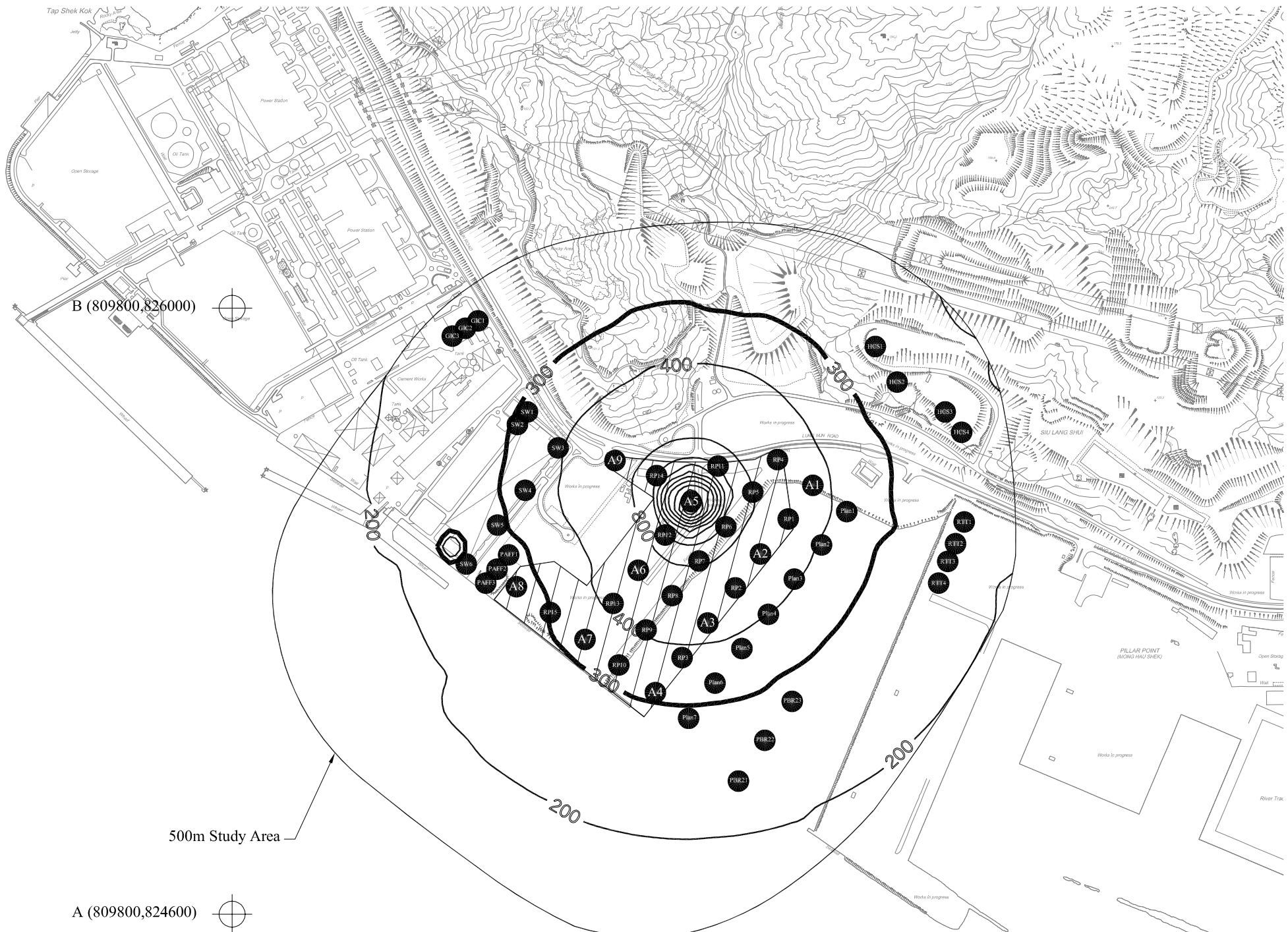
Figure 7-D6 Cumulative 1-hour NO 2 Concentration ( \mu\text{g}/\text{m}^3 ) at 61.5mPD emitted from Source Location A5 (Mitigated Scenario 2)
