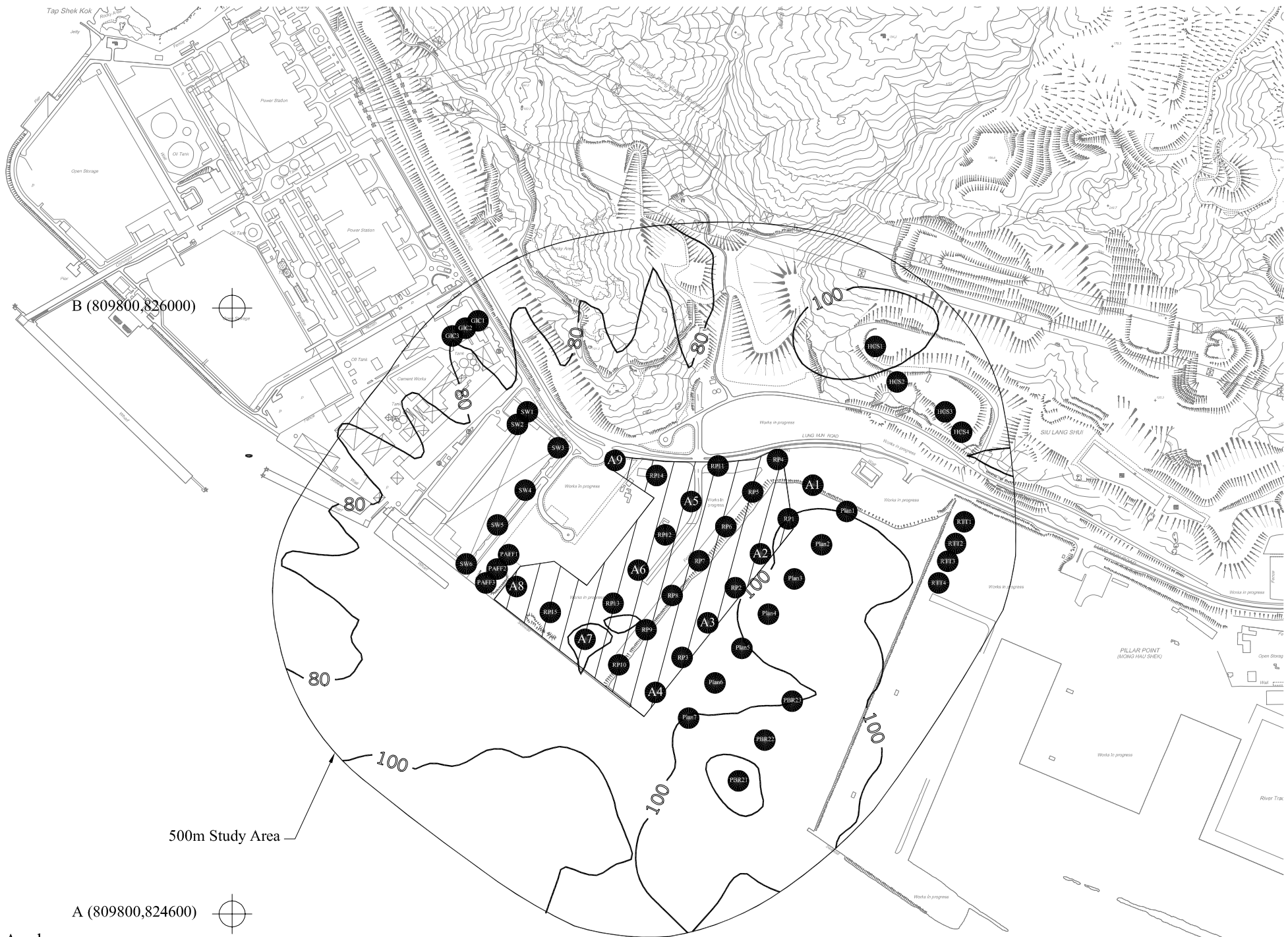
Figure 7-D1 Cumulative 1-hour NO 2 Concentration ( \mu\text{g}/\text{m}^3 ) at 8.5mPD emitted from Source Location A4 (Mitigated Scenario 2)
