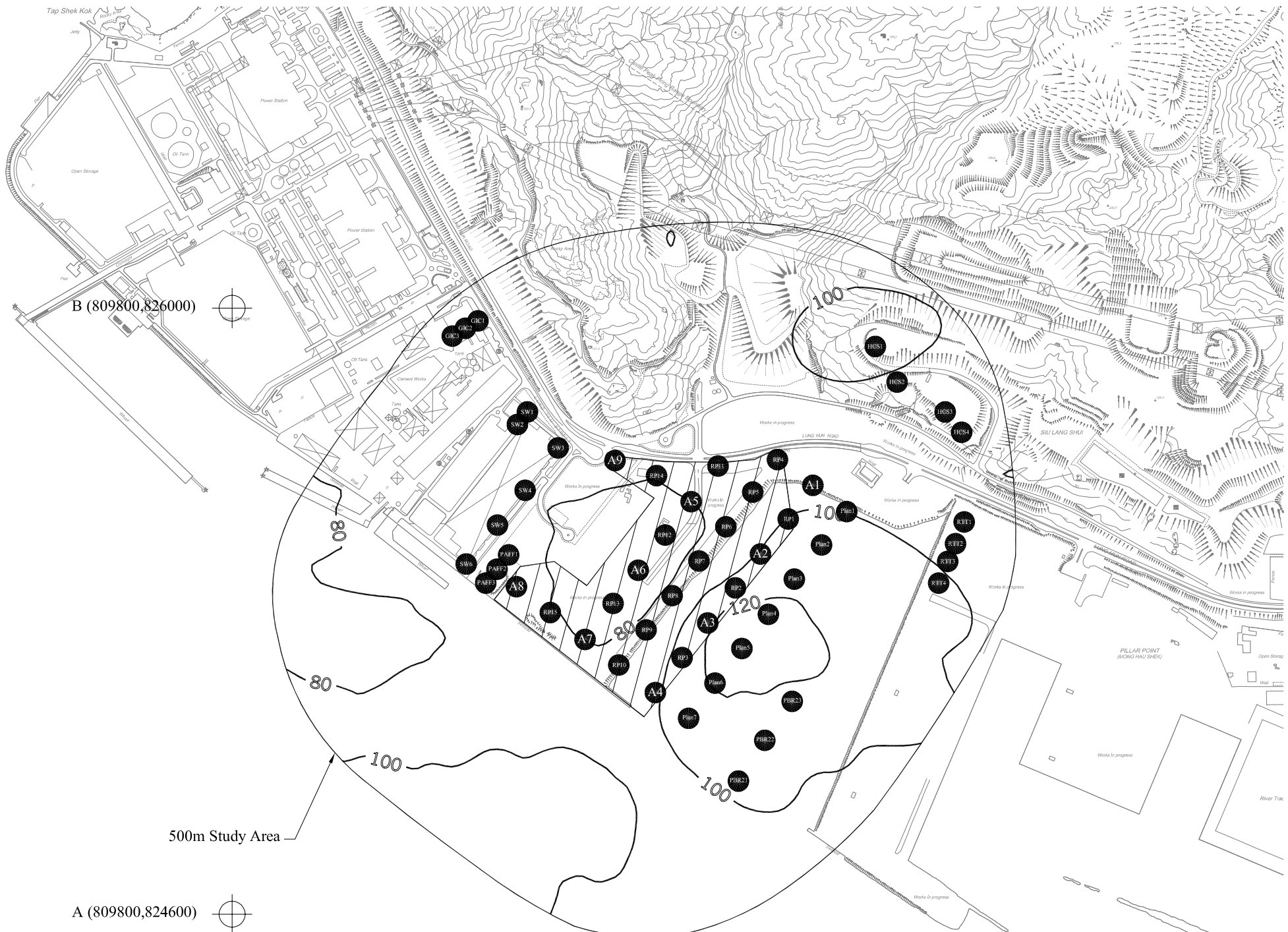
Figure 7-D2 Cumulative 1-hour NO 2 Concentration ( \mu\text{g}/\text{m}^3 ) at 8.5mPD emitted from Source Location A6 (Mitigated Scenario 2)
