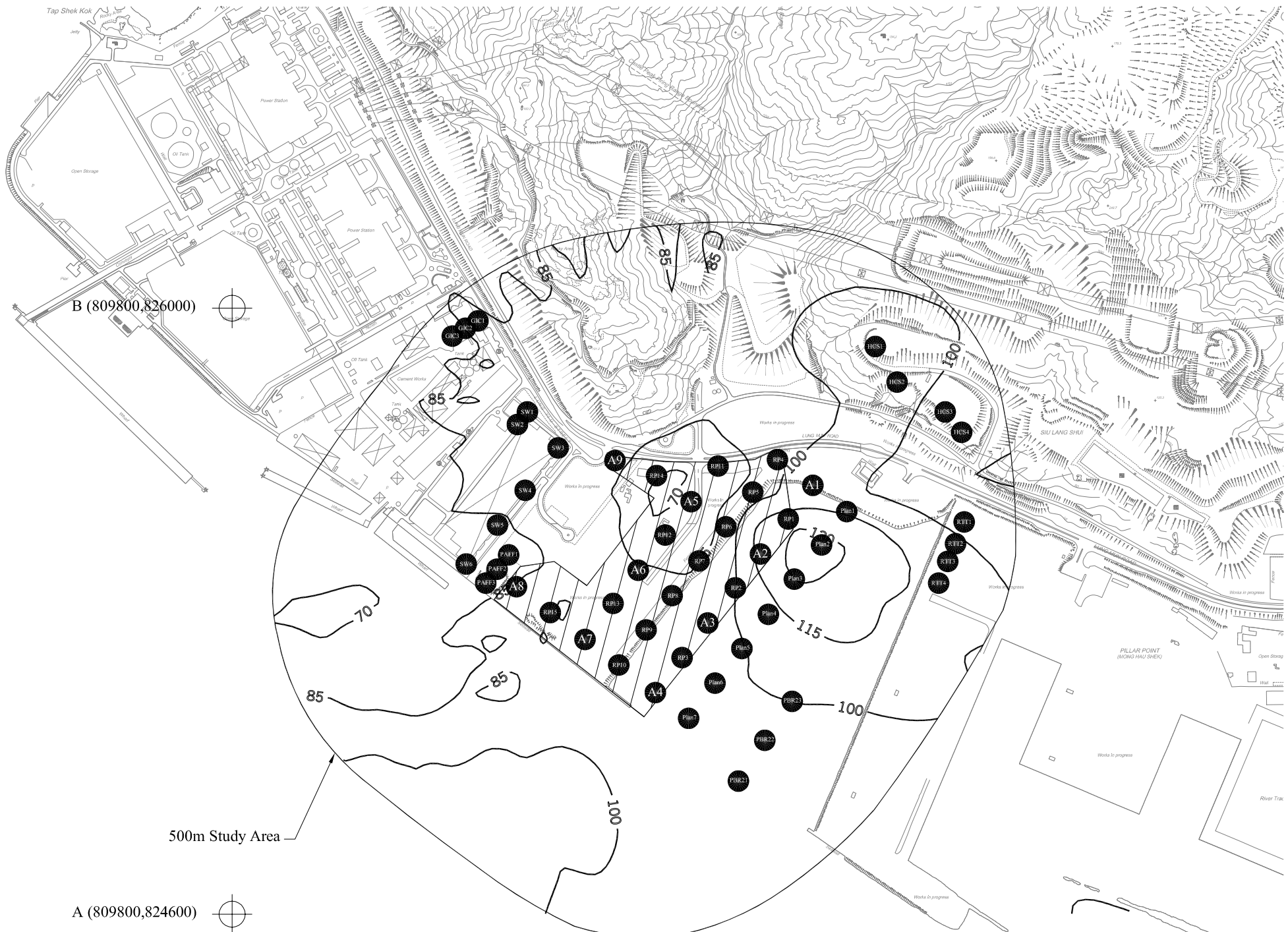
Figure 7-D4 Cumulative 1-hour NO 2 Concentration ( \mu\text{g}/\text{m}^3 ) at 22.5mPD emitted from Source Location A5 (Mitigated Scenario 2)
