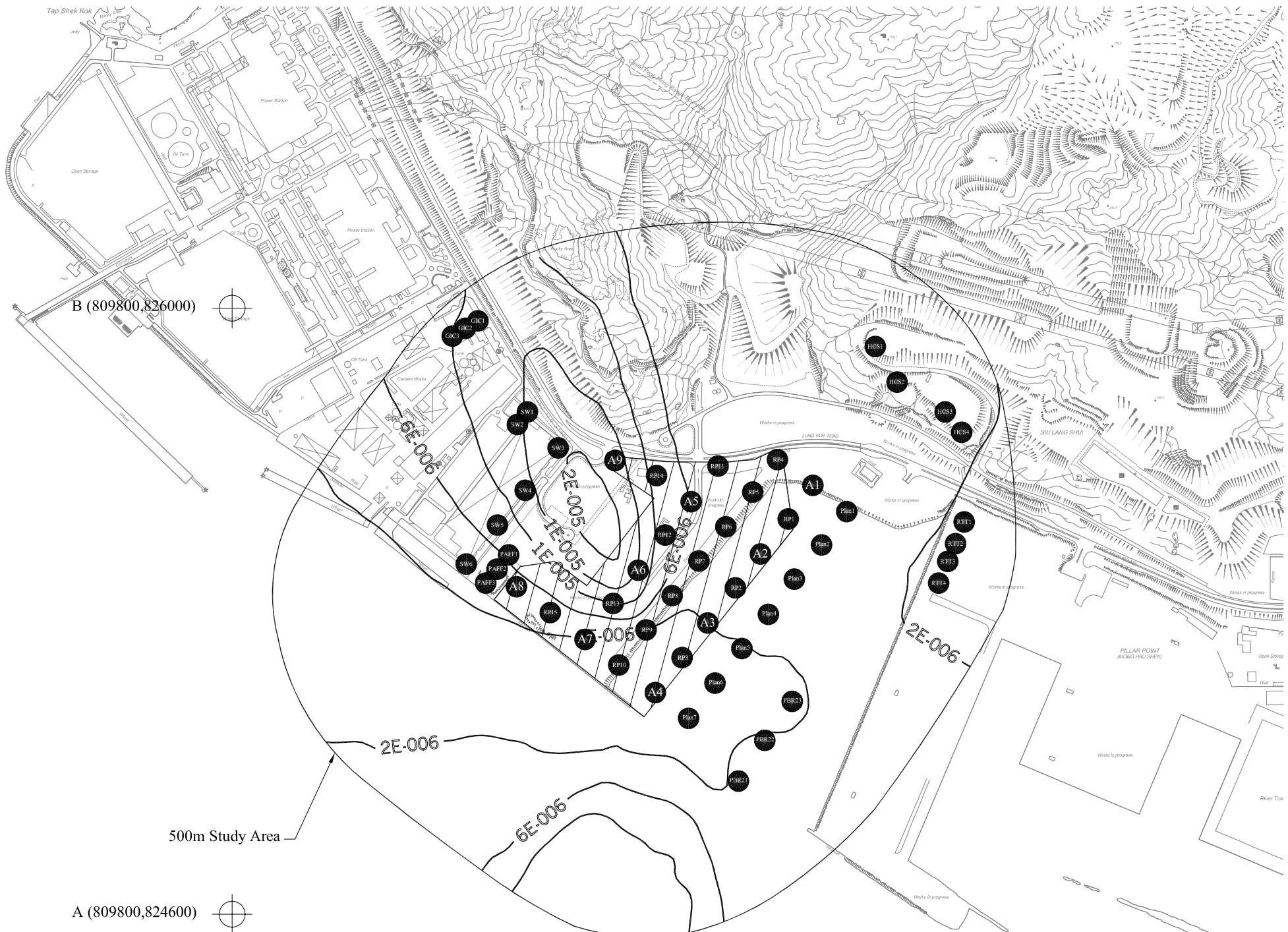
Scale: As shown Figure 7-F1 Cumulative Cancer Risk at 8.5mPD emitted from Source Location A4 (Mitigated Scenario 2)
