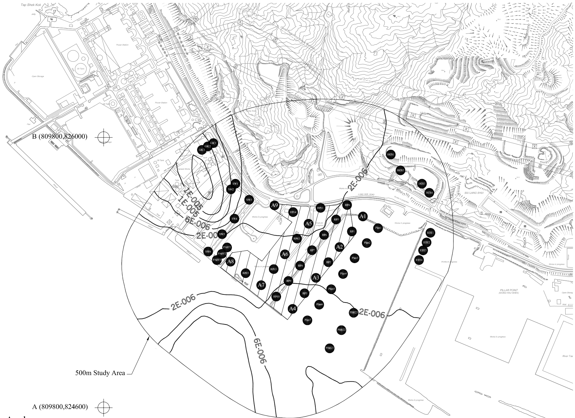
Scale: As shown Figure 7-F3 Cumulative Cancer Risk at 8.5mPD emitted from Source Location A8 (Mitigated Scenario 2)
