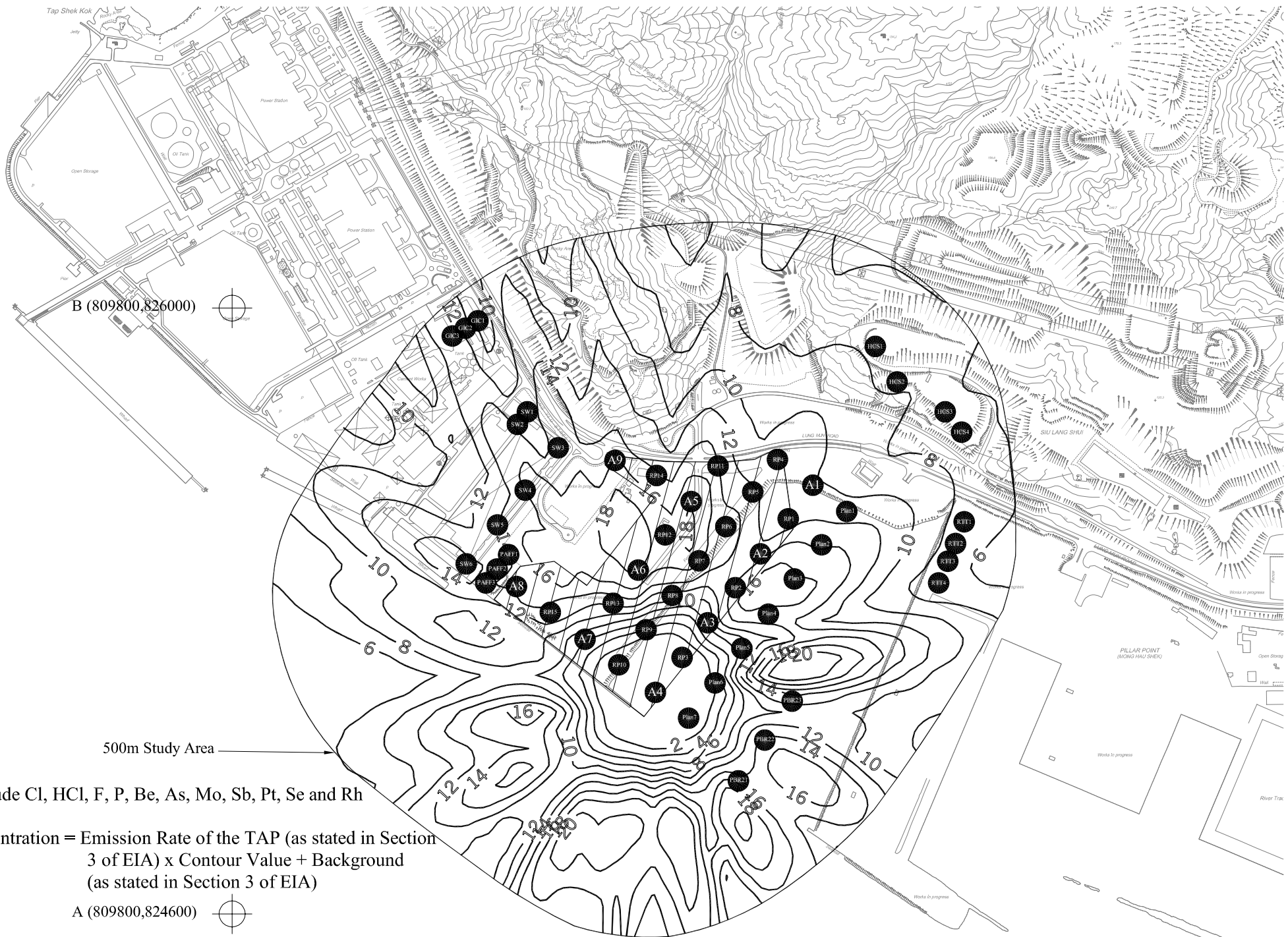
Figure B7-O1 Cumulative 4-hour TAPs Concentration ( \mu\text{g}/\text{m}^3 ) (with Emission Rate of 1 g/s) at 8.5mPD emitted from Source Location A4 (Mitigated Scenario 2)
