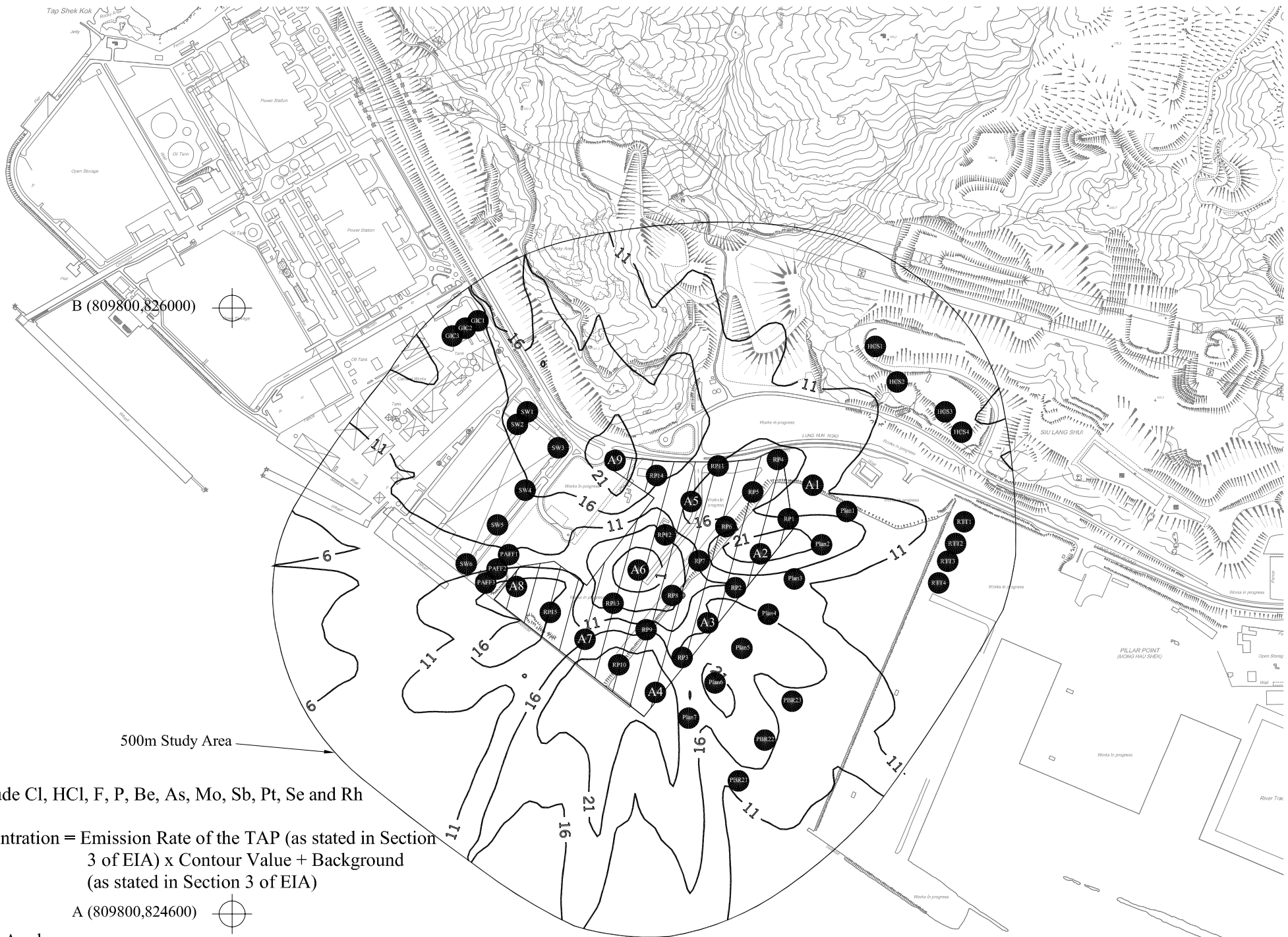
Figure 7-O4 Cumulative 4 Hour TAPs Concentration ( \mu\text{g}/\text{m}^3 ) at 22.5mPD emitted from Source Location A6 (Mitigated Scenario 2)
