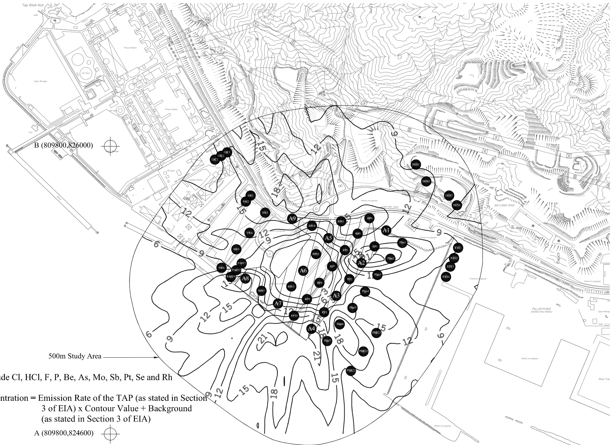
Figure B7-O2 Cumulative 4-hour TAPs Concentration ( \mu\text{g}/\text{m}^3 ) (with Emission Rate of 1 g/s) at 8.5mPD emitted from Source Location A6 (Mitigated Scenario 2)
