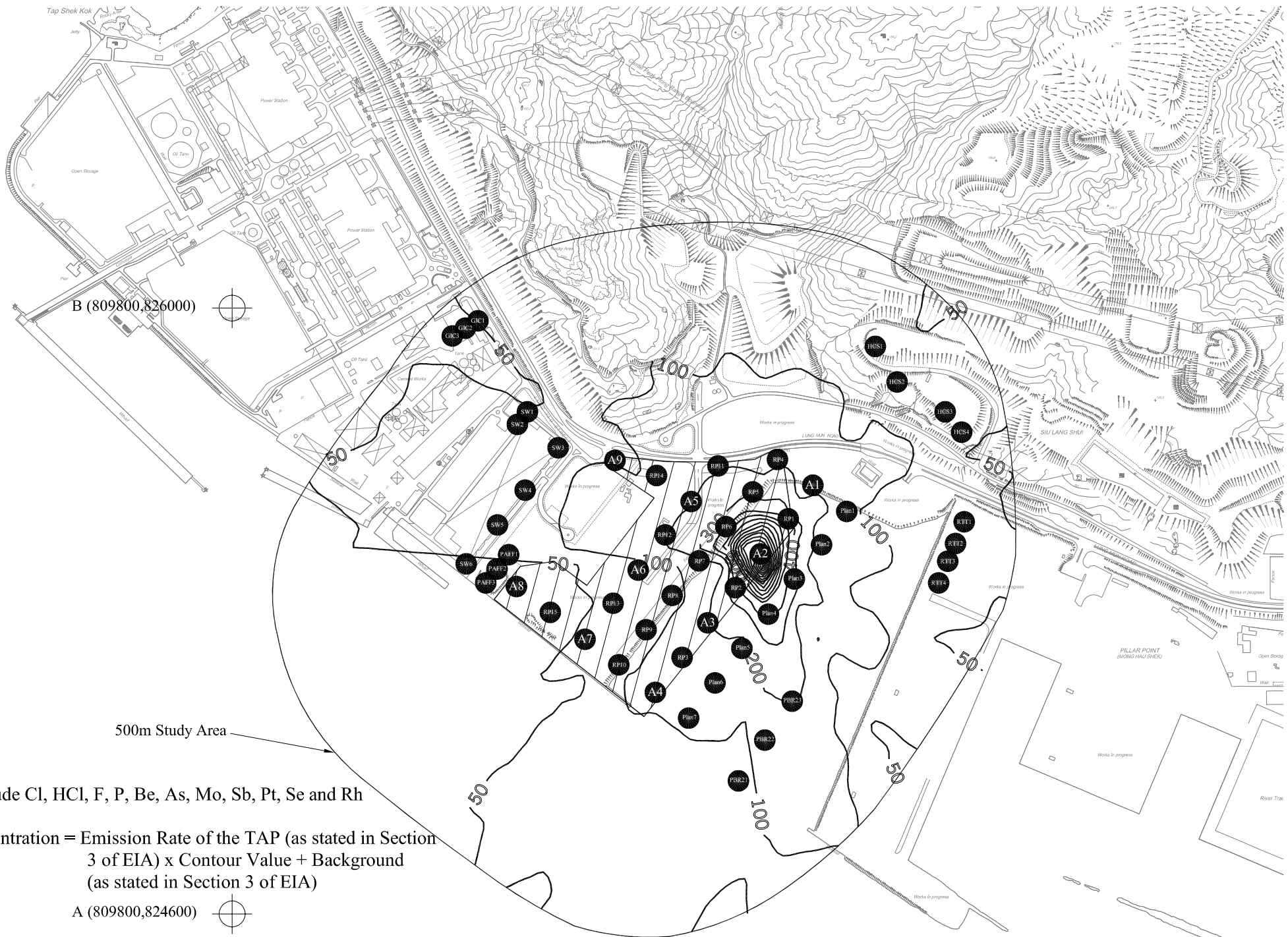
Figure B7-O5 Cumulative 4-hour TAPs Concentration ( \mu\text{g}/\text{m}^3 ) (with Emission Rate of 1 g/s) at 61.5mPD emitted from Source Location A2 (Mitigated Scenario 2)
