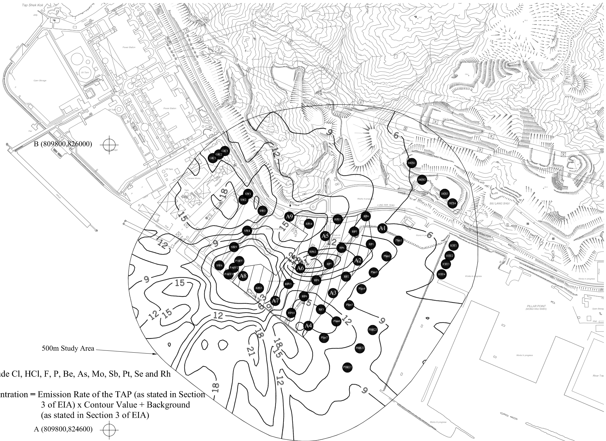
Figure B7-O3 Cumulative 4-hour TAPs Concentration ( \mu\text{g}/\text{m}^3 ) (with Emission Rate of 1 g/s) at 8.5mPD emitted from Source Location A8 (Mitigated Scenario 2)
