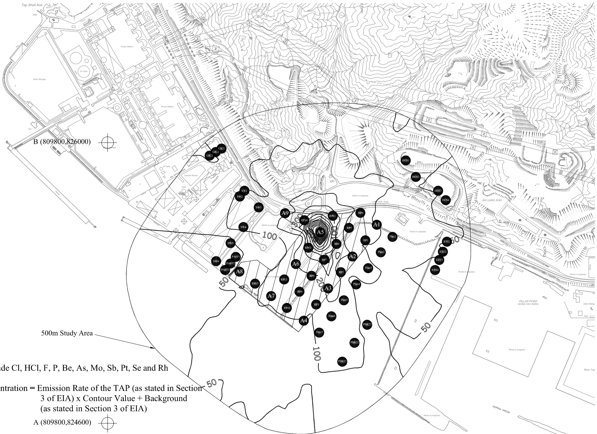
Figure B7-O6 Cumulative 4-hour TAPs Concentration ( \mu\text{g}/\text{m}^3 ) (with Emission Rate of 1 g/s) at 61.5mPD emitted from Source Location A5 (Mitigated Scenario 2)
