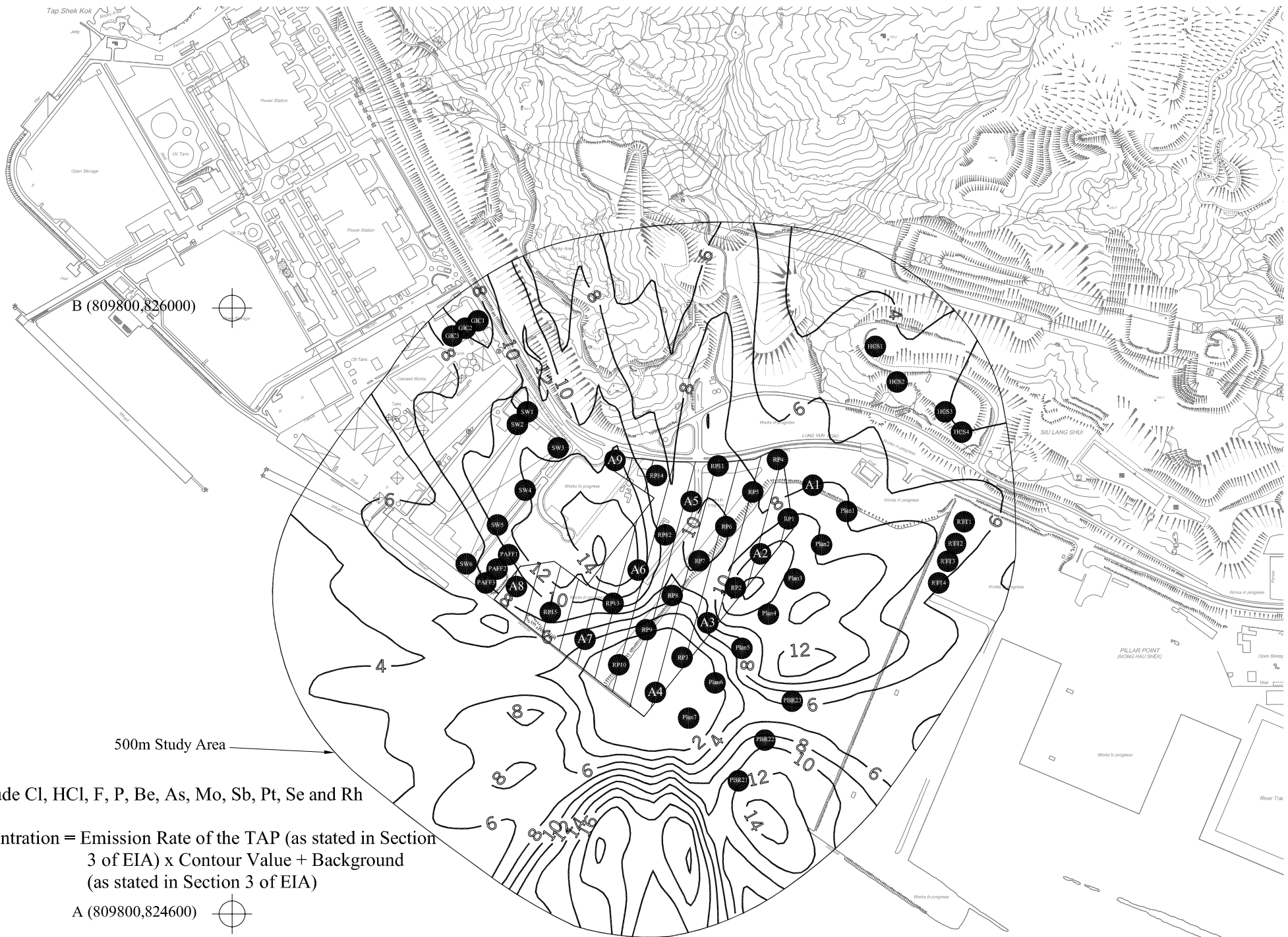
Figure B7-P1 Cumulative 8-hour TAPs Concentration ( \mu\text{g}/\text{m}^3 ) (with Emission Rate of 1 g/s) at 8.5mPD emitted from Source Location A4 (Mitigated Scenario 2)
