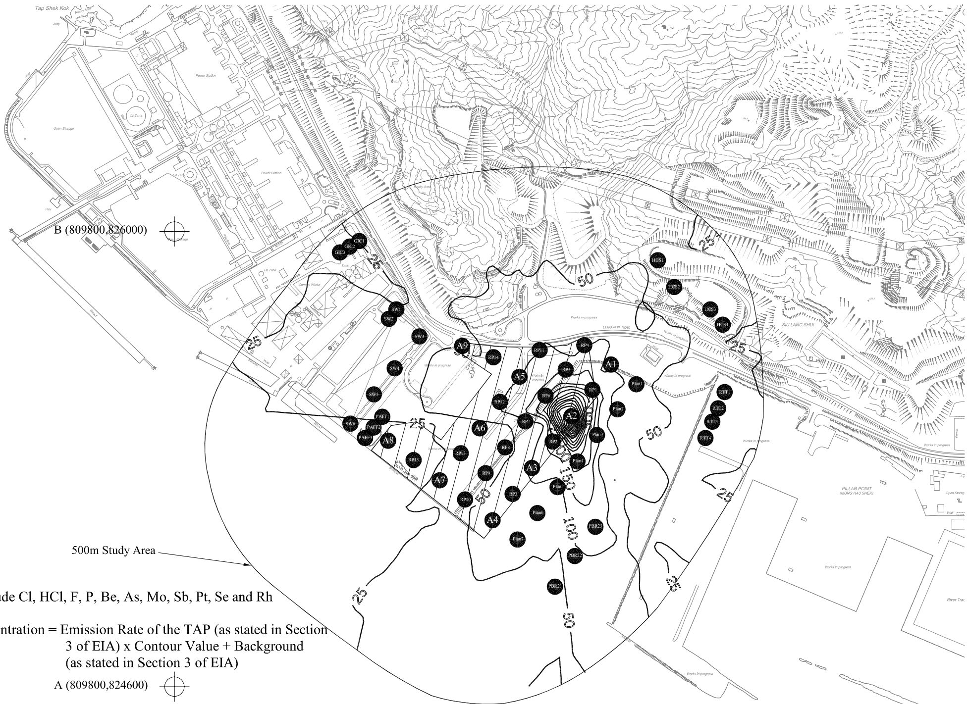
Figure B7-P5 Cumulative 8-hour TAPs Concentration ( \mu\text{g}/\text{m}^3 ) (with Emission Rate of 1 g/s) at 61.5mPD emitted from Source Location A2 (Mitigated Scenario 2)
