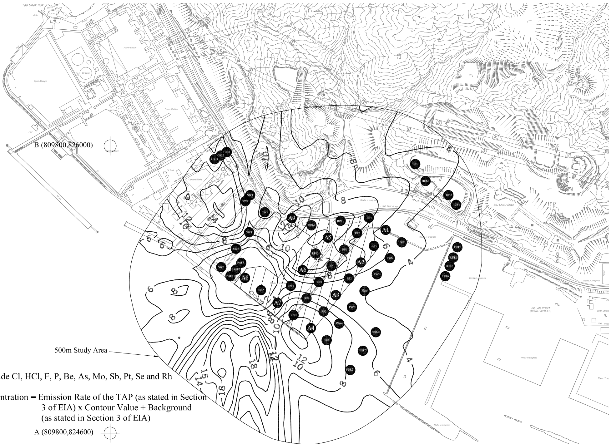
Figure B7-P3 Cumulative 8-hour TAPs Concentration ( \mu\text{g}/\text{m}^3 ) (with Emission Rate of 1 g/s) at 8.5mPD emitted from Source Location A8 (Mitigated Scenario 2)
