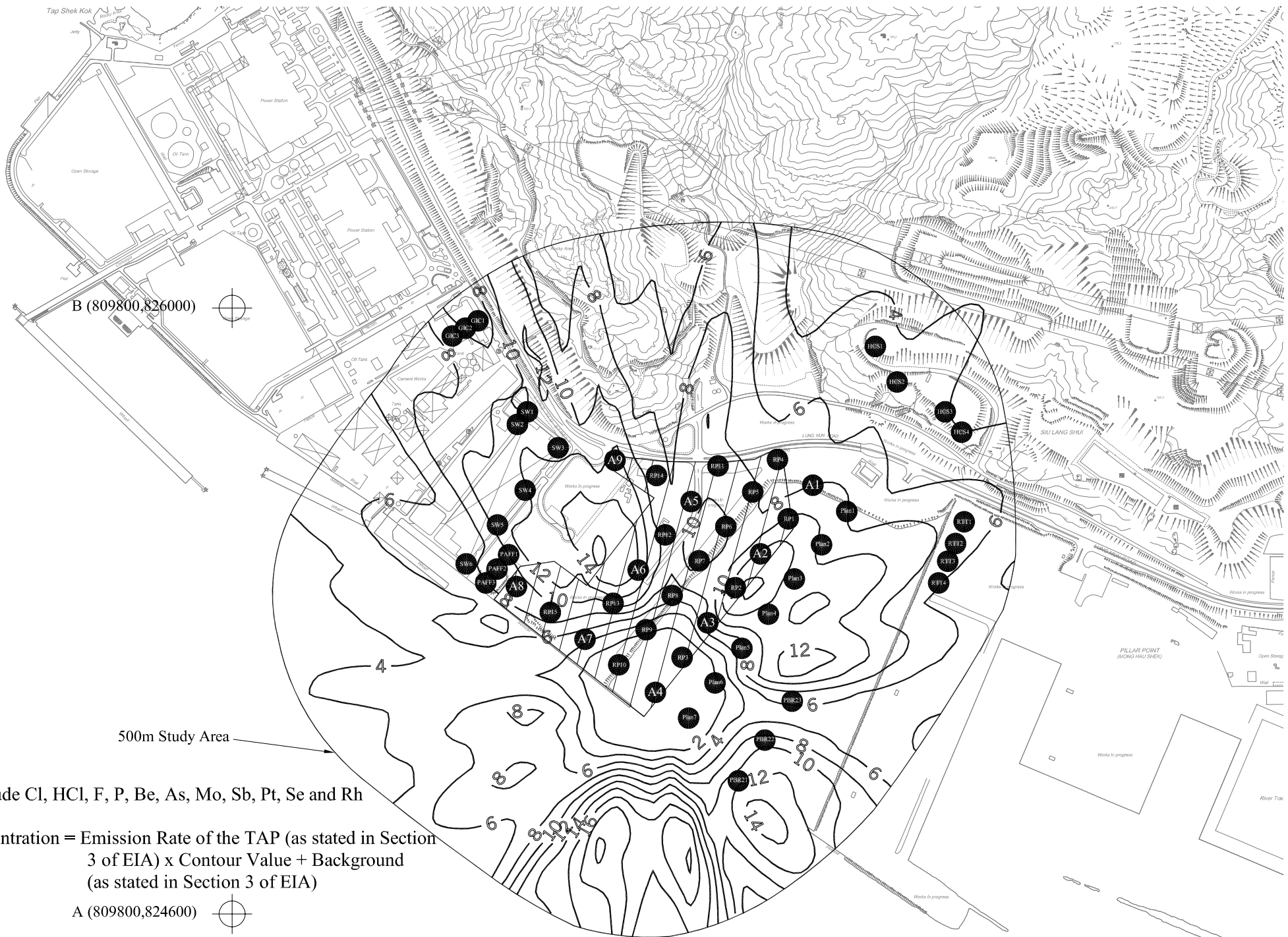
Figure B7-P2 Cumulative 8-hour TAPs Concentration ( \mu\text{g}/\text{m}^3 ) (with Emission Rate of 1 g/s) at 8.5mPD emitted from Source Location A6 (Mitigated Scenario 2)
