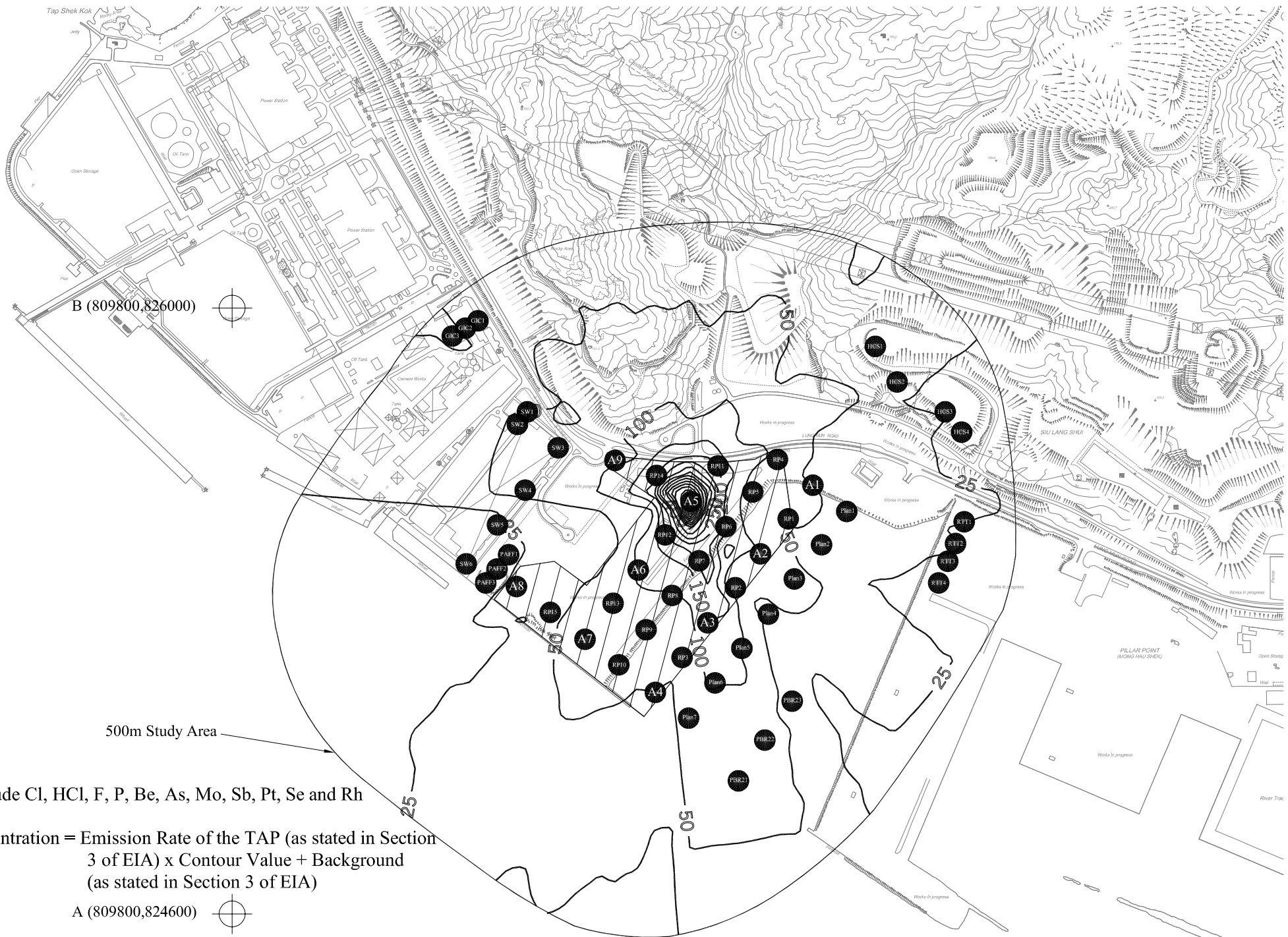
Figure B7-P6 Cumulative 8-hour TAPs Concentration ( \mu\text{g}/\text{m}^3 ) (with Emission Rate of 1 g/s) at 61.5mPD emitted from Source Location A5 (Mitigated Scenario 2)
