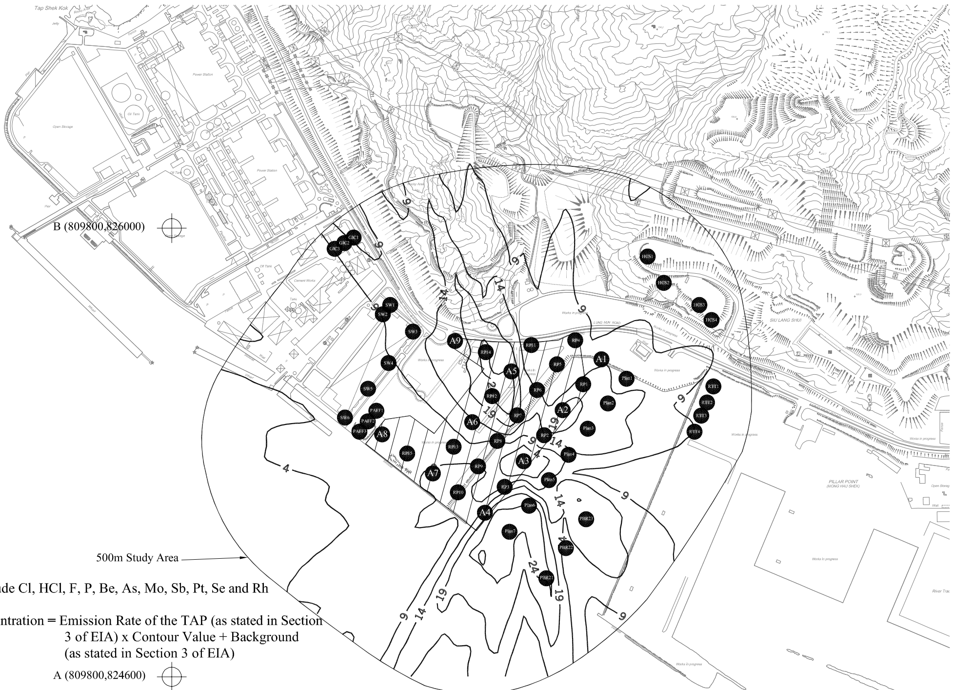
Figure 7-P4 Cumulative 8 Hour TAPs Concentration ( \mu\text{g}/\text{m}^3 ) at 22.5mPD emitted from Source Location A5 (Mitigated Scenario 2)
