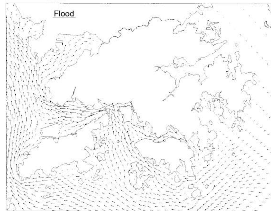
(b) Generalised Current Pattern in Hong Kong during Spring Tide in Winter
