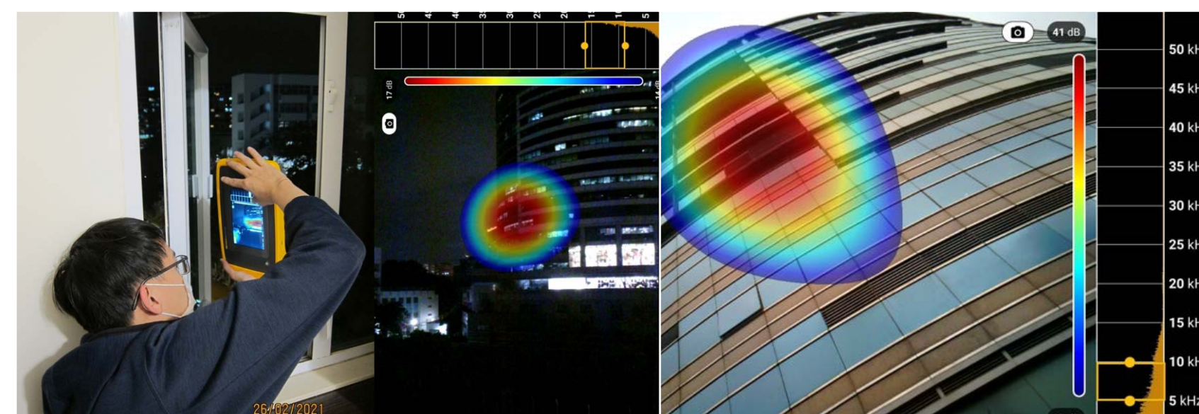
Dominant noise source identified by the "acoustic camera"
