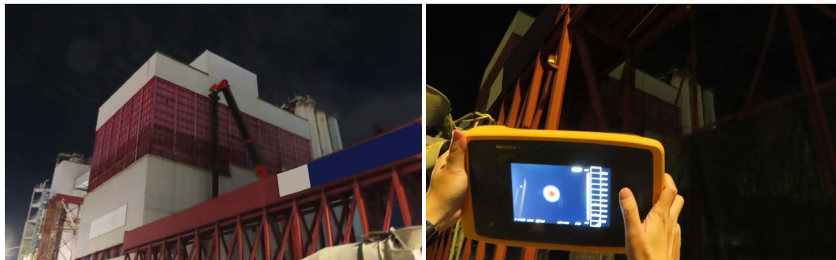
Identification of dominant noise source from multiple noise sources in alley
