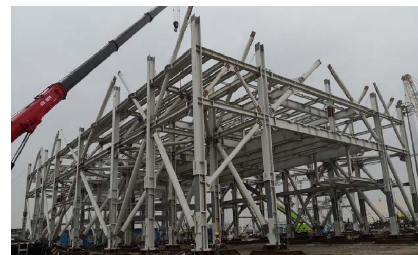
| Steel structure erection for prefabricated electrical and mechanical units at I-PARK1's Prefabrication Yard in Zhuhai (December 2021)
