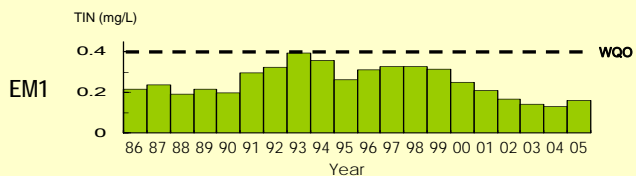
Total Inorganic Nitrogen (TIN) (depth-averaged)
