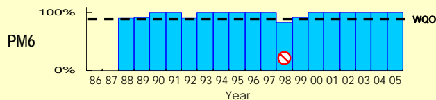
Dissolved Oxygen (DO) (depth-averaged)
