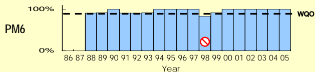
Dissolved Oxygen (DO) (bottom)
