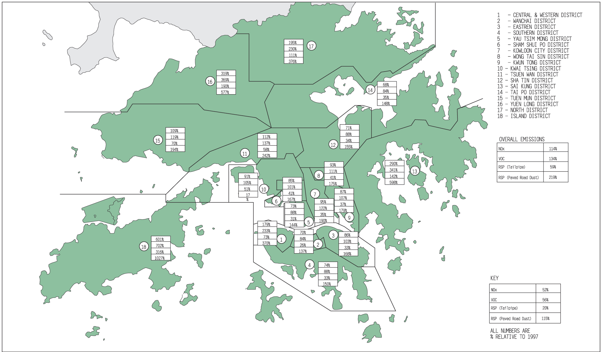
Third Comprehensive Transport Study (CE 84/96) POLLUTANT EMISSIONS IN 2016 RELATIVE TO 1997 BY DISTRICTS 2016 RECOMMENDED TRANSPORT STRATEGY HIGH GROWTH SCENARIO (HIGH END)
