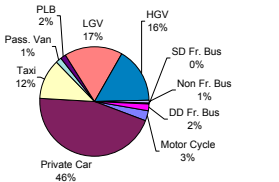
Annual vkt By Vehicle Classifications
