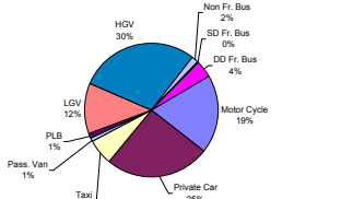
Annual VOC By Vehicle Classifications
