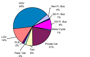
Annual NOx By Vehicle Classifications
