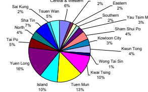
Annual RSP (tailpipe) By District
