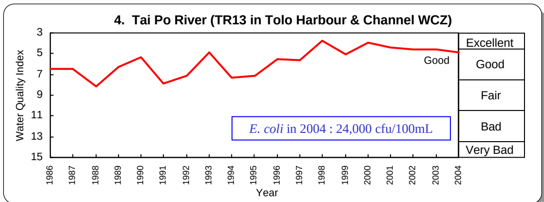
Figure 3-a: Water Quality Index (WQI) & E. coli levels of the major rivers in Hong Kong
