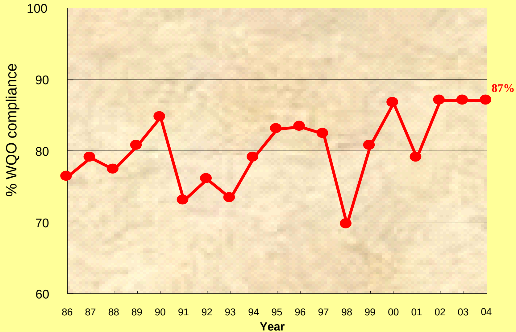
Figure 4 Overall compliance with marine Water Quality Objectives in Hong Kong, 1986 - 2004
