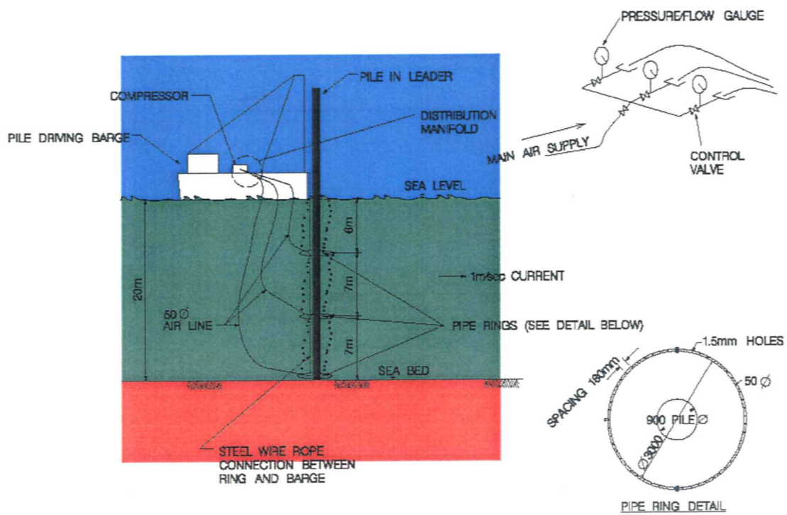
Figure 2 Canadian Bubble Jacket
