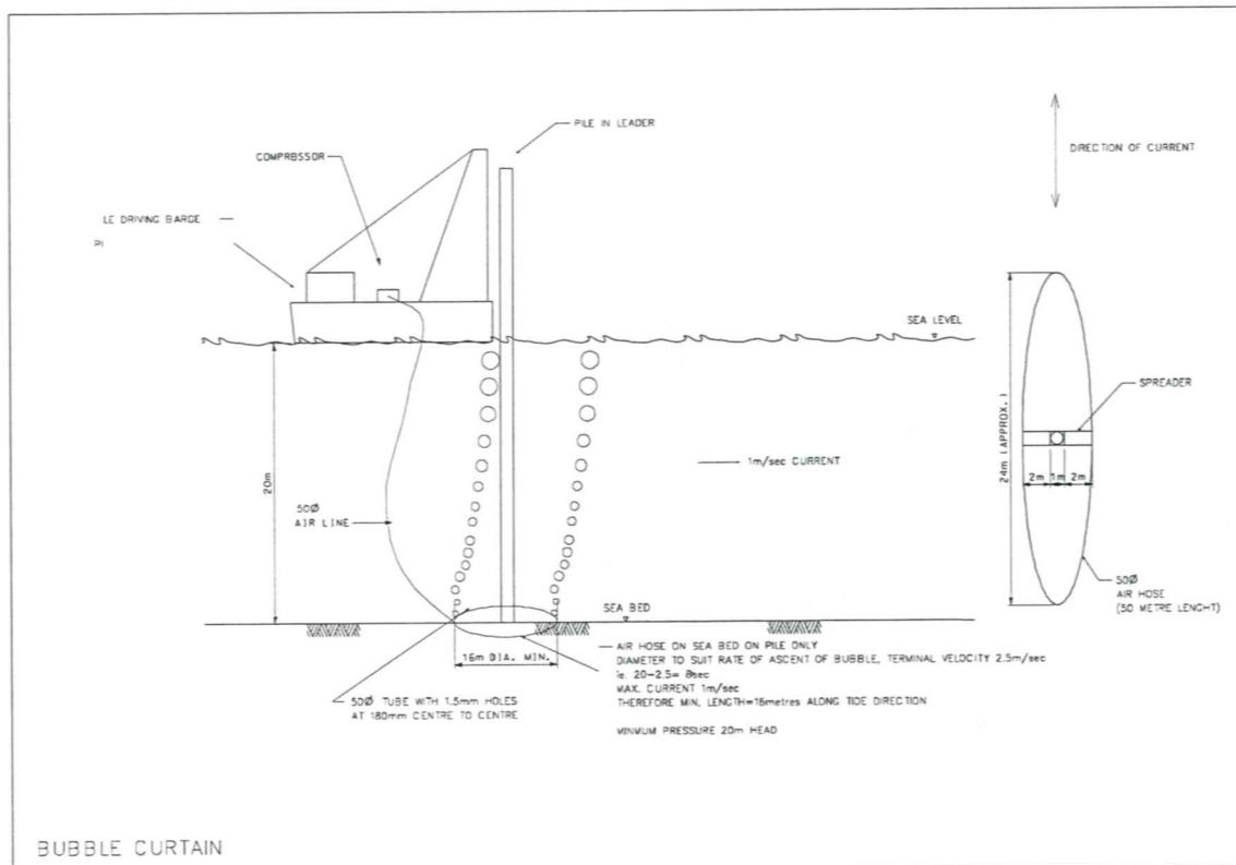
Figure 4 Bubble Curtain
