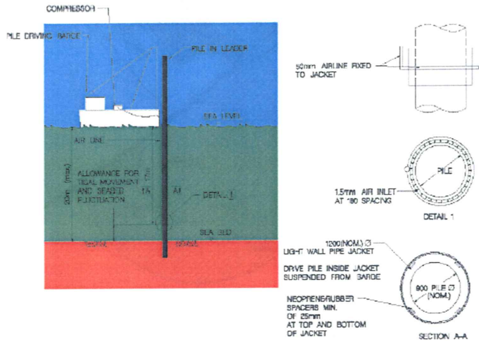
Figure 4 Bubble Curtain
