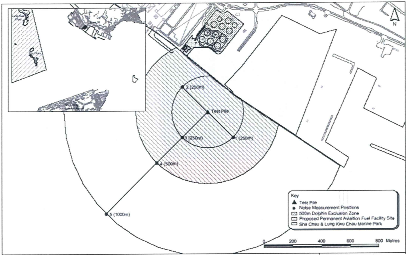
Figure 1 PAFF Jetty Location and Noise Monitoring Points
