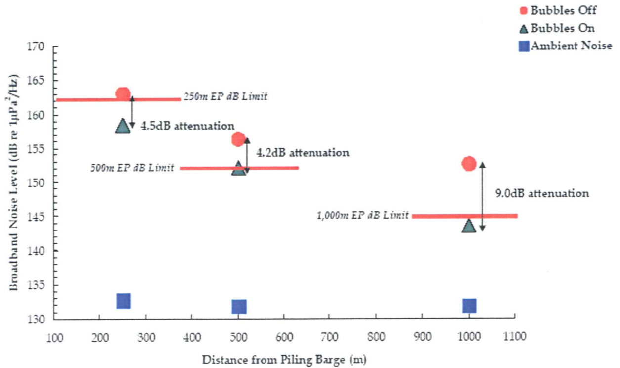
Figure 6 Broadband Noise Mitigation (EIA Dolphin Sensitive Range 400 Hz to 12.8 kHz) Achieved by Option 7 at all Distances from the Test Pile
