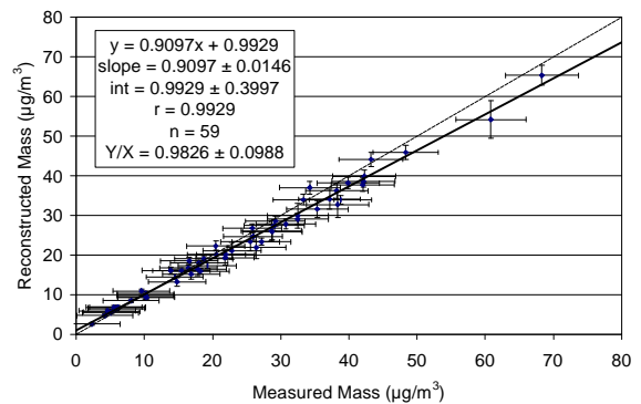
Figure 3-9. Scatter plots of reconstructed mass versus measured mass from \text{PM}_{2.5} data acquired at: a) all three sites; b) the MK site; c) the TW site; and d) the HT site.
