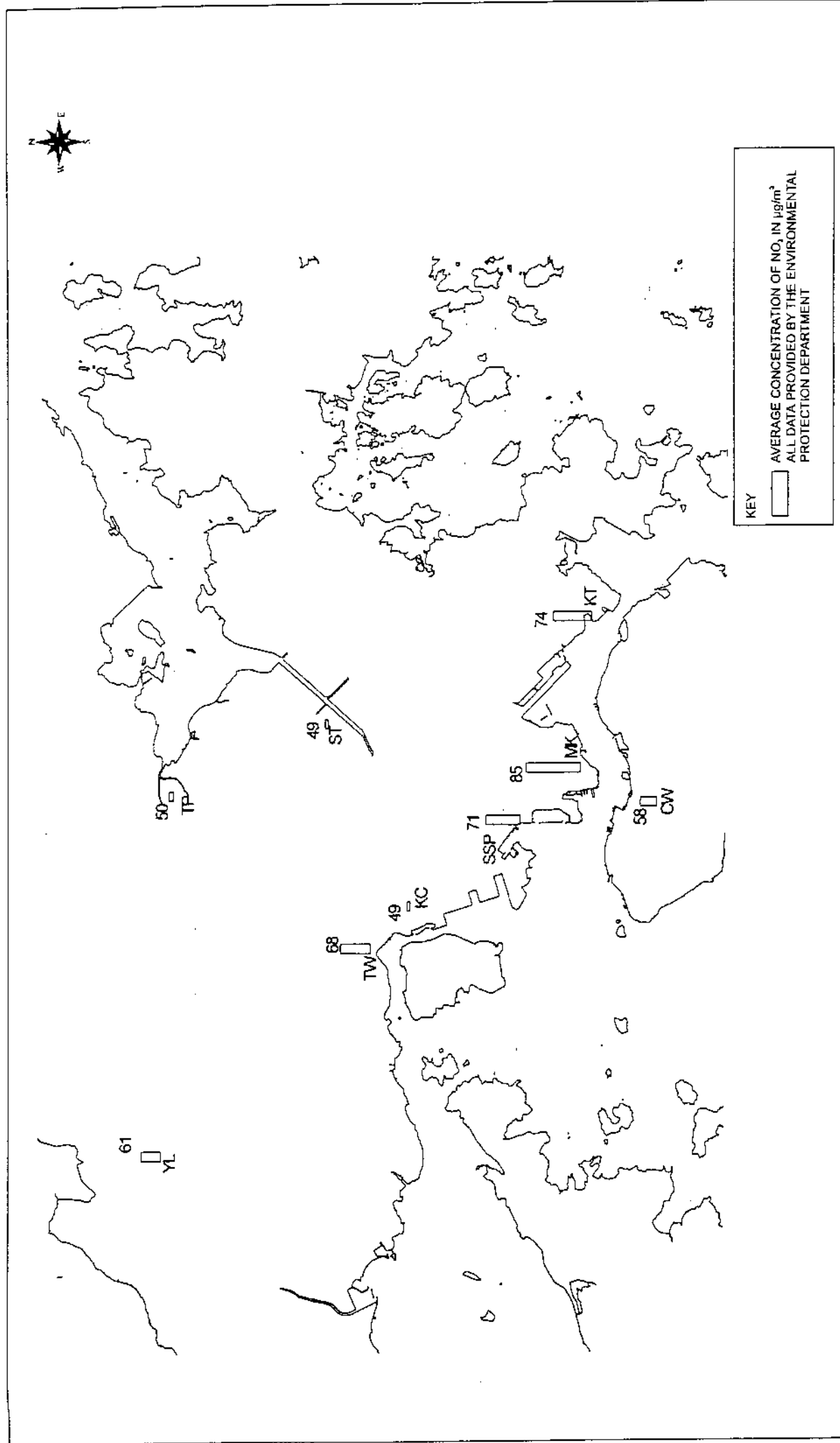
Third Comprehensive Transport Study (CE 84/86) ANNUAL AVERAGE NITROGEN DIOXIDE CONCENTRATIONS
