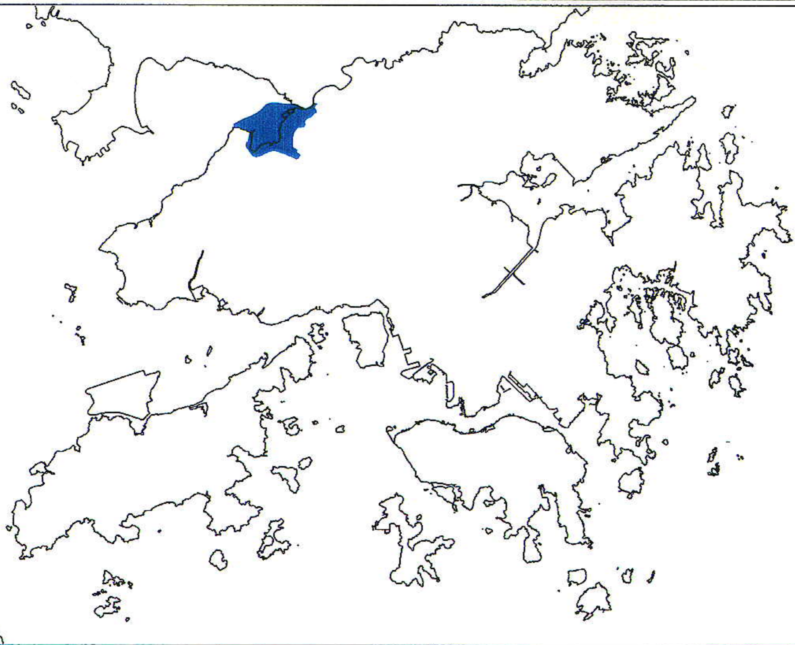
FIGURE 3.3f Ramsar Site
