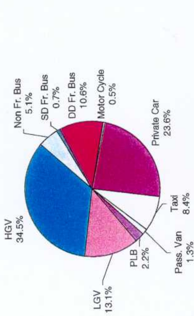
Annual NOx By Vehicle Classifications (1997)
