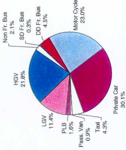
Annual VOC By Vehicle Classifications (1997)
