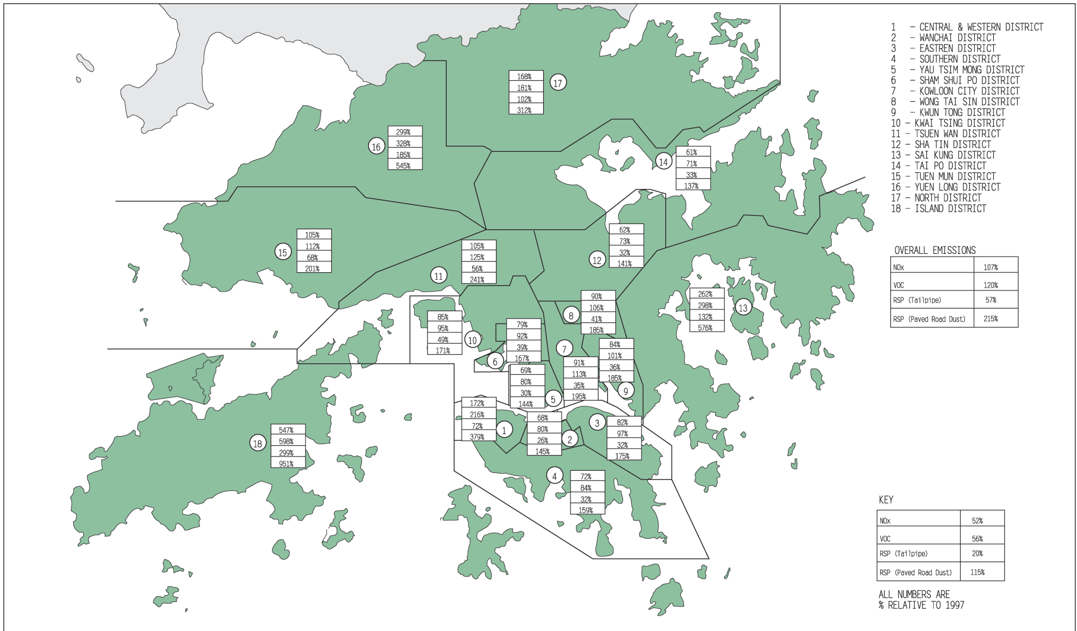
Third Comprehensive Transport Study (CE 84/96) POLLUTANT EMISSIONS IN 2016 RELATIVE TO 1997 BY DISTRICTS 2016 RECOMMENDED TRANSPORT STRATEGY HIGH GROWTH SCENARIO (LOW END)
