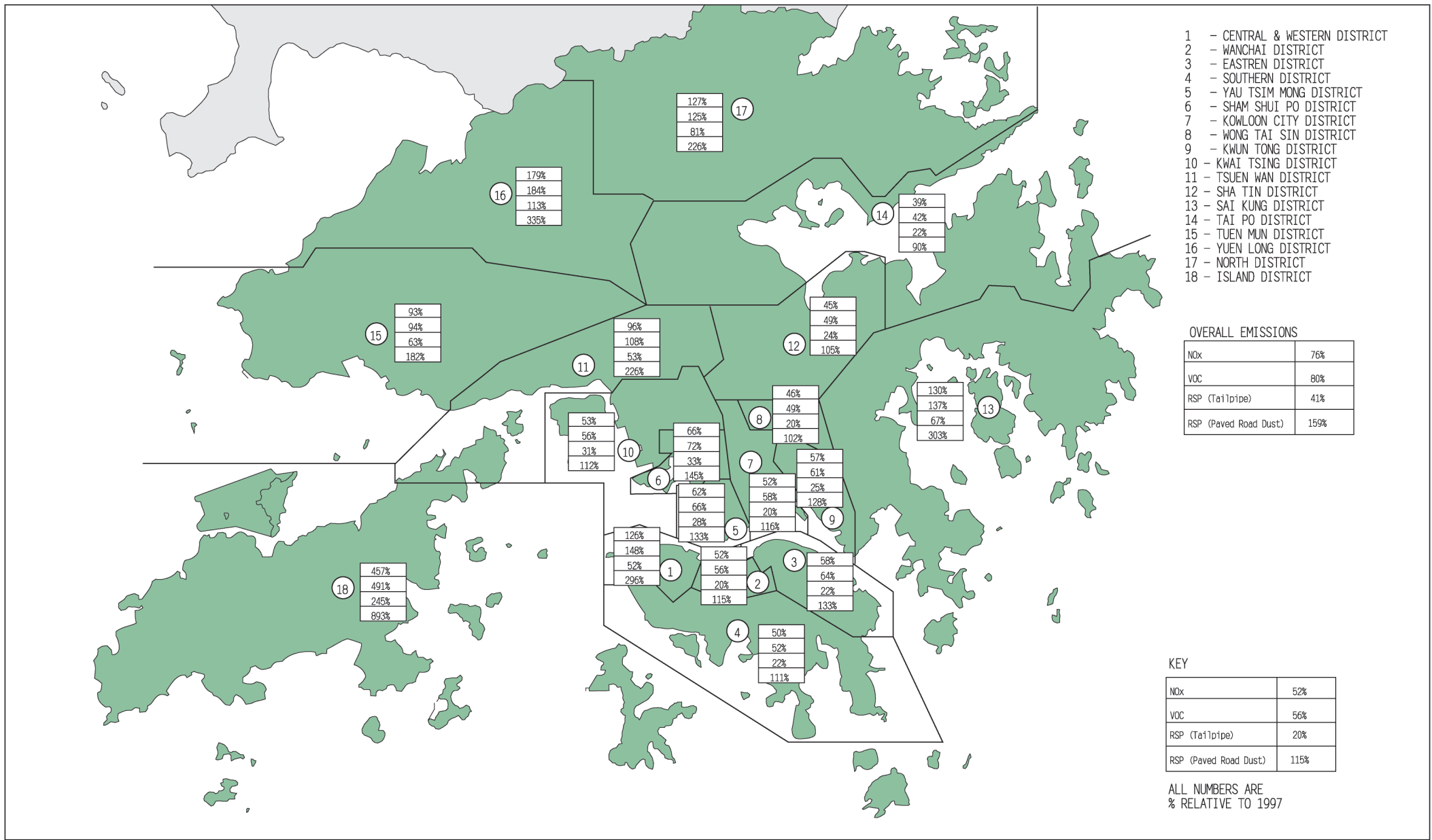
Third Comprehensive Transport Study (CE 84/96) POLLUTANT EMISSIONS IN 2016 RELATIVE TO 1997 BY DISTRICTS 2016 RECOMMENDED TRANSPORT STRATEGY (LOW GROWTH SCENARIO)
