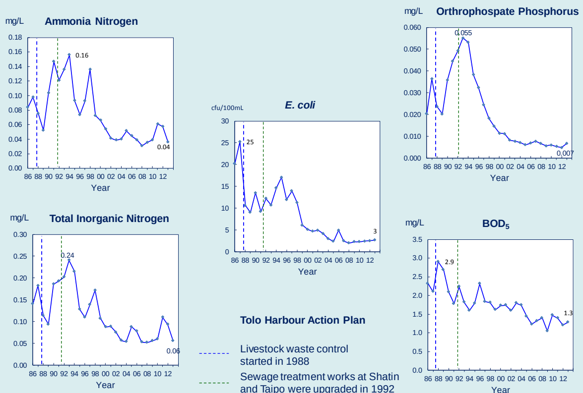
Water quality changes in Tolo Harbour and Channel WCZ, 1986-2013
