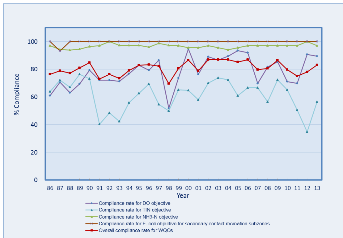
Overall compliance rate with the WQOs and the compliance rates for the four objectives in Hong Kong, 1986-2013
