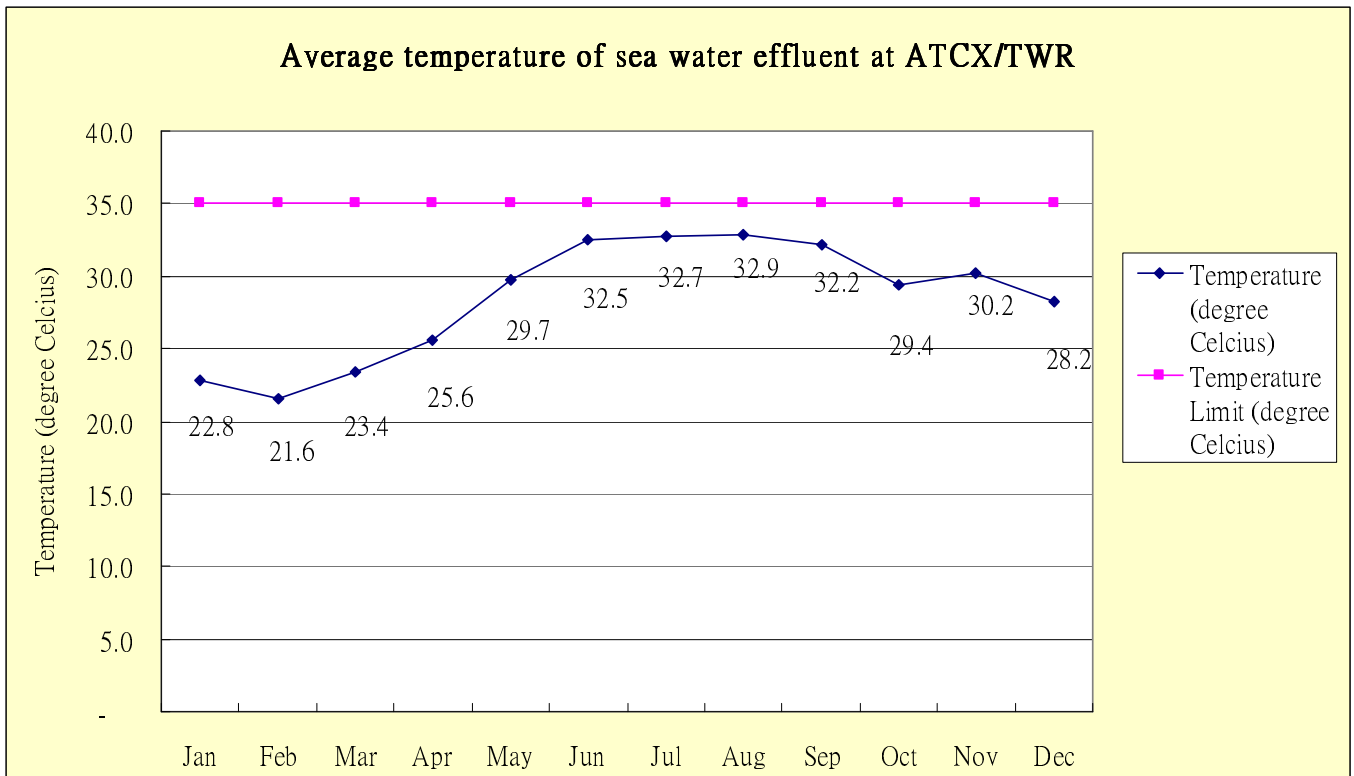
Figure 17: Average temperature of sea water effluent at ATCX/TWR
