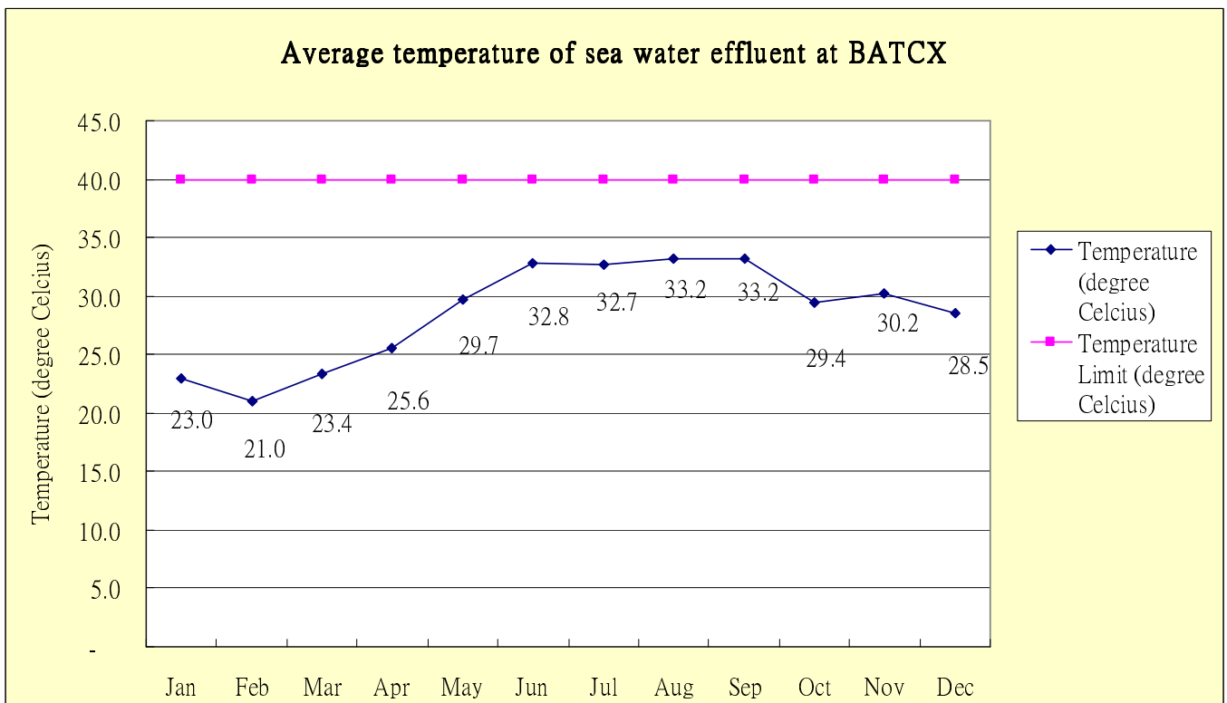
Figure 18: Average temperature of sea water effluent at BATCX
