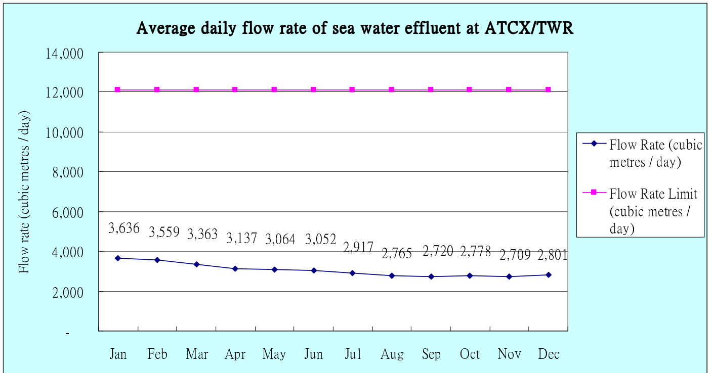
Figure 15: Average daily flow rate of sea water effluent at ATCX/TWR
