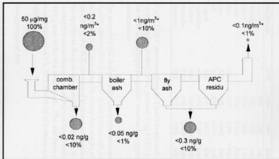
Figure 5.5b Concentrations (TE) and Balance of PCDD/PCDF in an modern MSW Incinerator. (% = proportion of total inventory input to the system.) * = raw gas concentration
