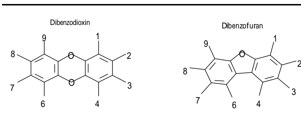
Figure 2.1a Basic Structure of PCDDs and PCDFs
